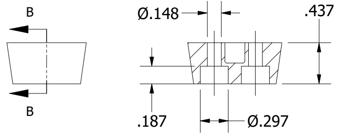
SECTION B-B SCALE 1 : 1
