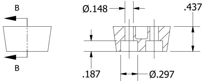
SECTION B-B SCALE 1 : 1
